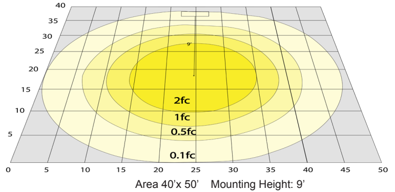
Area 40'x 50' Mounting Height: 9'
